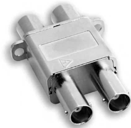
FULL SIZE PATCH-JACK 75Ω TERMINATED & NON-TERMINATED
