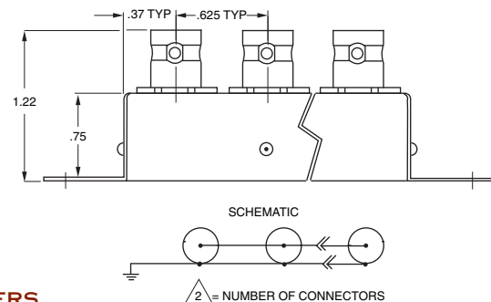
ADAPTERS MULTIPLE PARALLEL NETWORK 50Ω MPN- \triangle /BNC 50Ω MPN- \triangle /TNC Contact the factory for more information.
