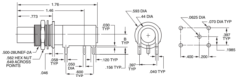
CIRCUIT BOARD BULKHEAD MOUNTING MINI-WECO PATCH JACK 75Ω RIGHT ANGLE LONG LEG VERSION CBBJR12 B = .24 CBBJR12A B = .34 Mounting Hole: D3.250
